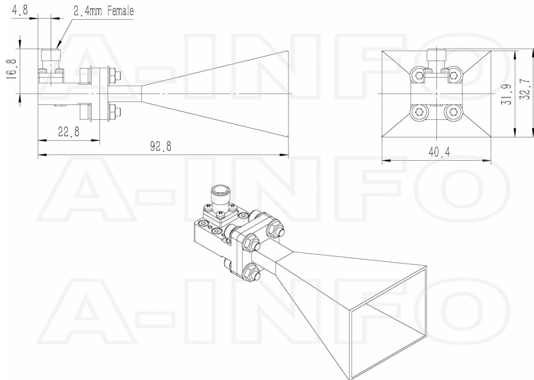
2.4mm-Female Output (P/N: LB-28-20-64-C-2.4F)
